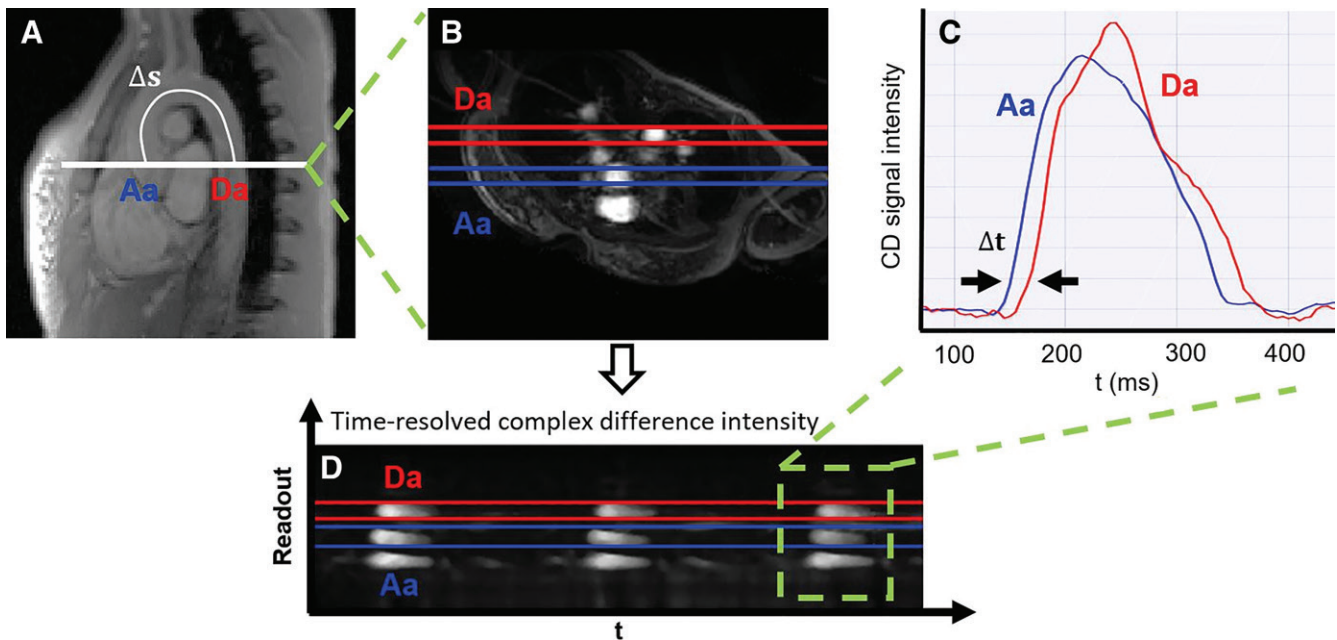
Figure 4: Measurement of aortic pulse wave velocity. A, Sagittal view of the aortic arch with path length of the flow wave between the ascending aorta (Aa) and descending aorta (Da; \Delta s ). B, Axial view showing Aa and Da, and the time course of the, C, complex difference (CD) signals during three cardiac cycles. D, CD signal intensity averaged across the aorta width during a single cardiac cycle (the transit time [t] is indicated). Sample data shown for a representative participant. t = time.
