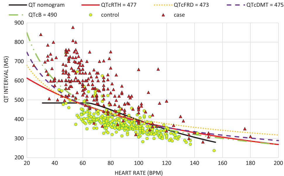
Figure 2. QTcRTH vs. QTcFRD vs. QTcDMT vs. QTcBZT vs. nomogram.
